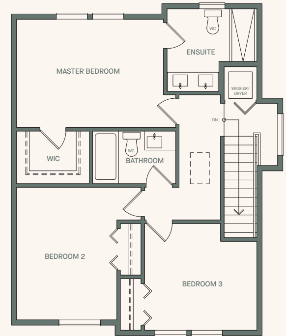
Third Floor
